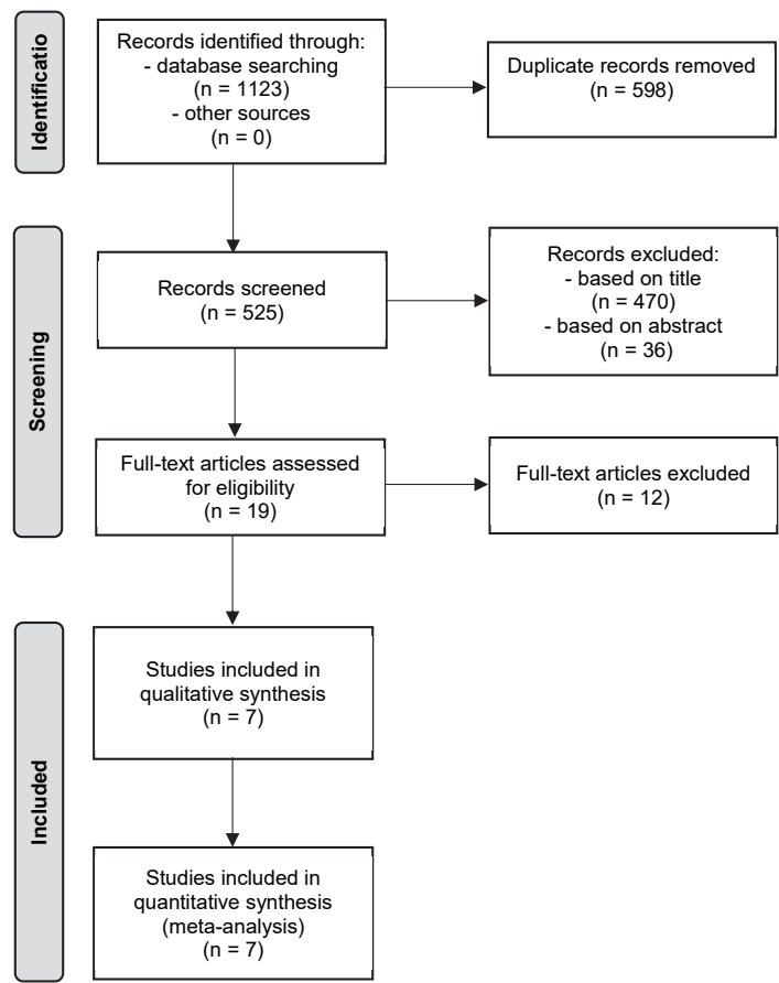
Figure 1. PRISMA flowchart
