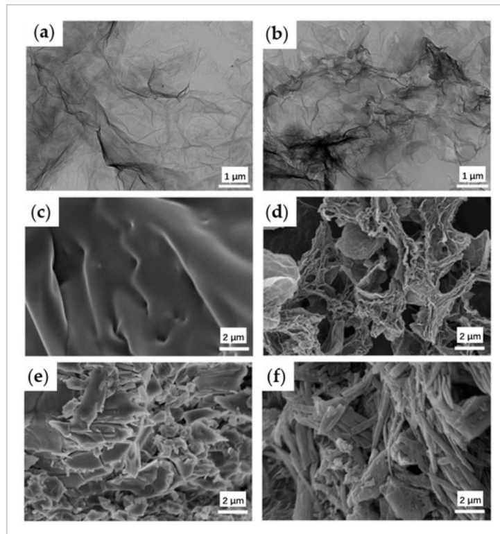
Figure 21. The process of functionalizing and immobilizing substrates on the GO surface in a photoelectrochemical (PEC) lipase sensor. TEM analysis of (a) GO and (b) 3DGO; SEM analysis of (c) GO-ITO, (d) 3DGO-ITO, (e) PNb-3DGO-ITO, and (f) GDH-PNb-3DGO-ITO. Reproduced from [241] under the terms of the CC-BY Creative Commons Attribution License, copyright 2022 Elsevier Ltd.
