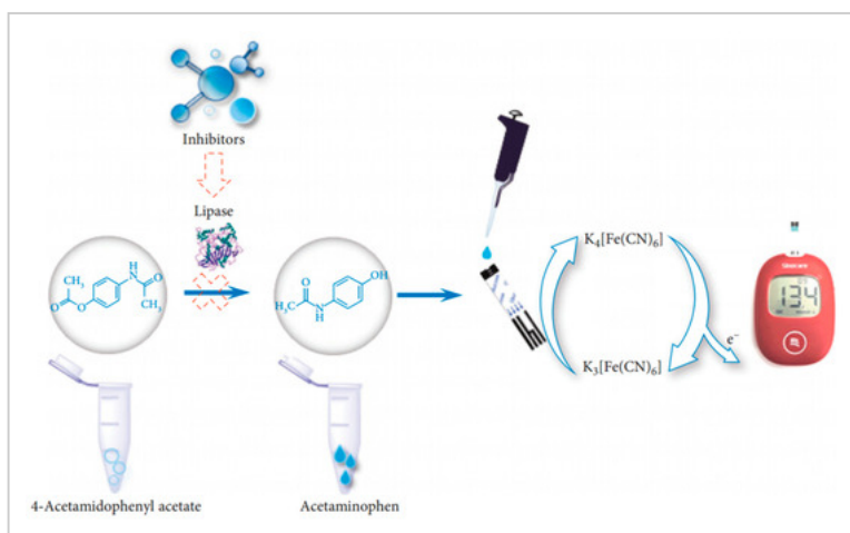
Figure 22. Portable lipase assay. Electrochemical sensing using a glucose meter. Reproduced [243] from under the terms of the CC-BY Creative Commons Attribution License, copyright 2022 Hindawi Ltd.
