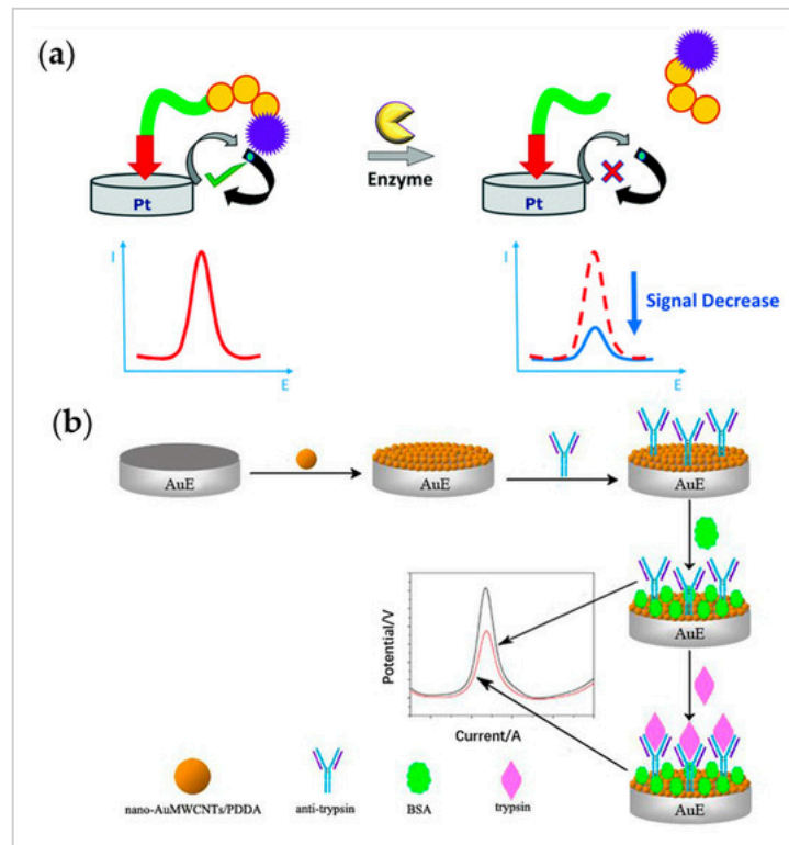
Figure 17. Principles of electrochemical methods for the detection of trypsin. (a) Hydrolysis of the immobilized substrate using trypsin. Reproduced from [188] under the terms of the CC-BY Creative Commons Attribution License, copyright 2022 by the Royal Society of Chemistry. (b) Anti-trypsin antibody specifically binds to trypsin. The black curve in the graph shows the results in the absence of trypsin. With the addition of trypsin, the signal is shown as a red
