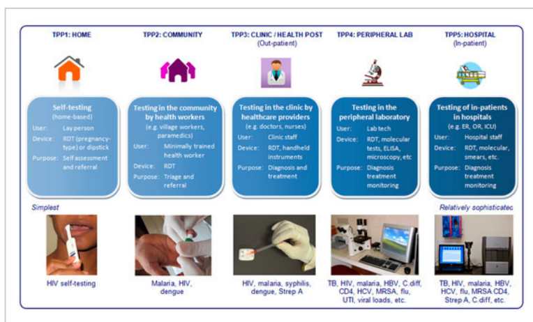
Figure 3. Diversity of target product profiles, users, and settings within the spectrum of Point-of-Care testing. Reproduced from [48] under the terms of the CC-BY Creative Commons Attribution License, copyright 2012 Public Library Science.
