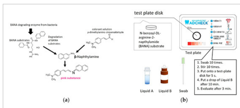
Figure 19. Convenient protease self-sensing method. (a) The mechanism of ADCHECK to detect TLP activity. (b) Components of the ADCHECK kit. Reproduced from [220] under the terms of the CC-BY Creative Commons Attribution License, copyright 2022 MDPI.
