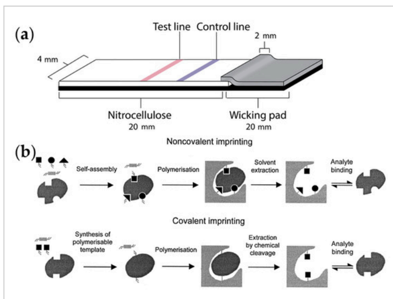
Figure 11. Some special methods. (a) Antigen test strips that were widely used during the COVID-19 outbreak. Reproduced from [119] under the terms of the CC-BY Creative Commons Attribution License, copyright 2020 American Chemical Society. (b) Molecularly imprinted polymers for sensing molecules. Reproduced with permission from [120], copyright 2000 by American Chemical Society.
