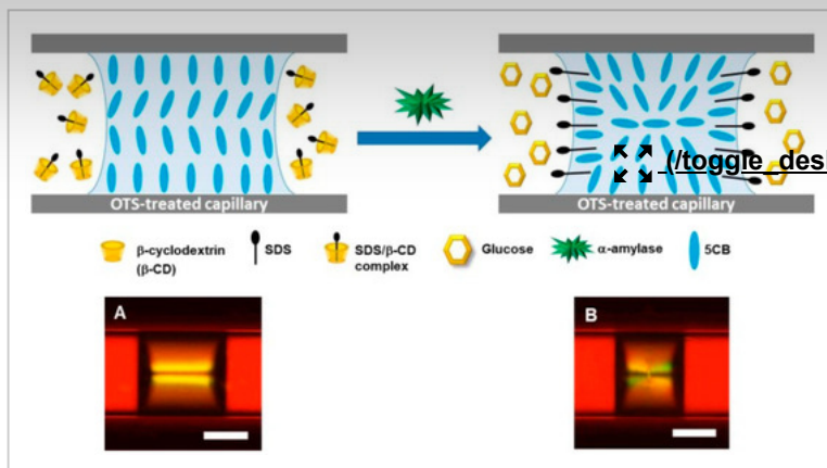
Figure 7. The hydrolysis of the substrate by amylase affects the arrangement of the liquid crystal molecules, showing different patterns. (A) Two bright lines indicate the planar orientation of the LC at the LC-aqueous interface after adding a synthetic \beta -CD/SDS solution, (B) four petal-shaped texture indicates a switch to the homeotropic orientation after the addition of a \alpha -amylase hydrolyzed solution of \beta -CD/SDS. Scale bar = 200 \mu m. Reproduced with permission from [83], copyright 2020 by Elsevier Ltd.
